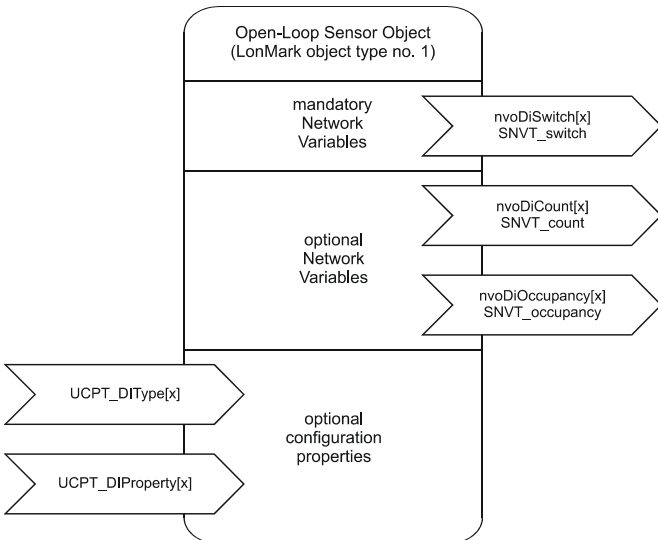
Fig. 3. Profile of LONMARK sensor objects for DIs
