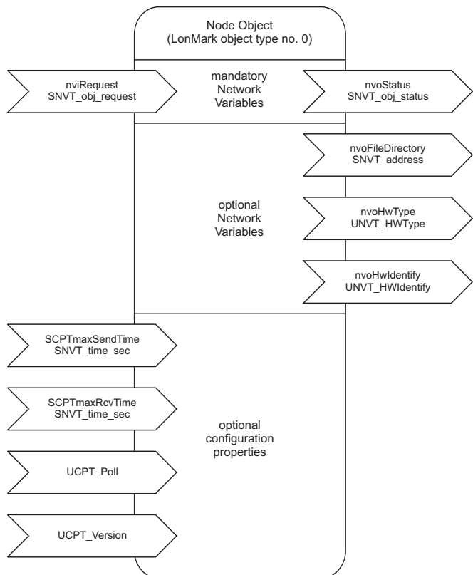
Fig. 1. Profile of LONMARK Node Object
