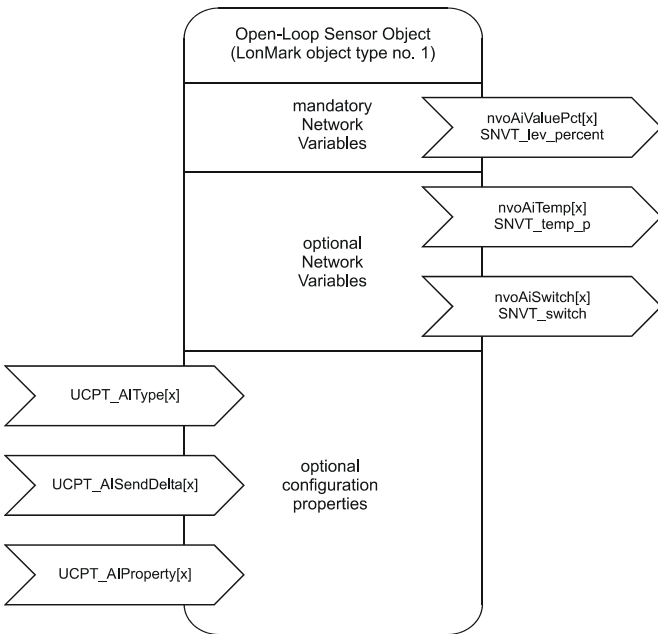
Fig. 2. Profile of LONMARK sensor object for UIs
