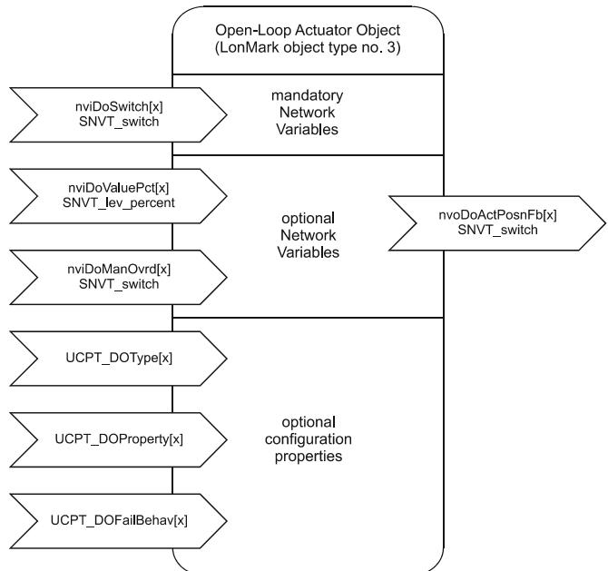
Figure 5. Profile of LONMARK actuator objects for relays
